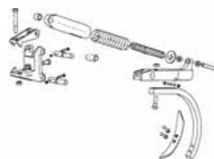
Tine and hitch CH-100
