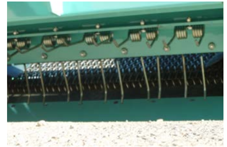
Spikes of the frontal roller
